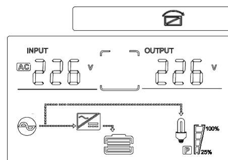
Fig. 4-4 Panel de control en modo bypass
